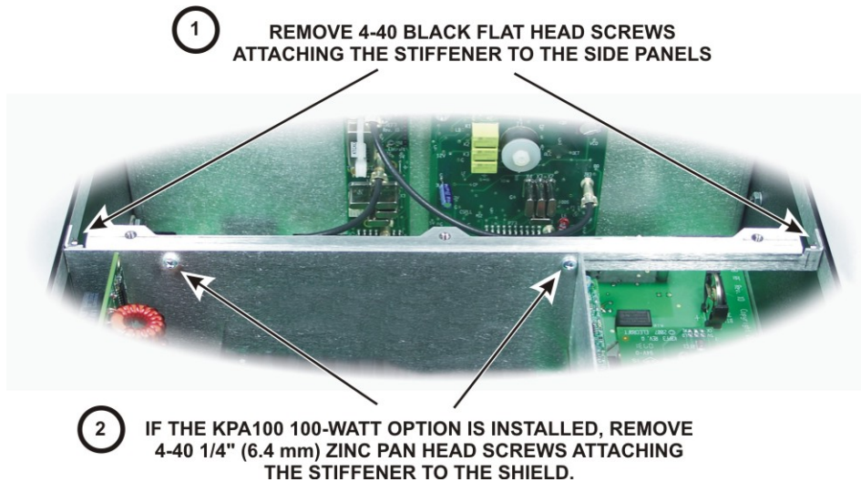
Figure 3. Removing the Chassis Stiffener Bar.
