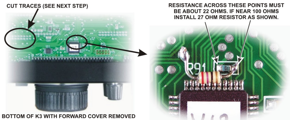
Figure 22. R91 Modification.
