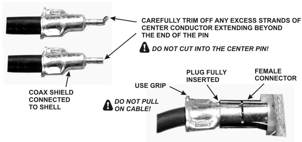
Figure 27. TMP Cable Connectors.
